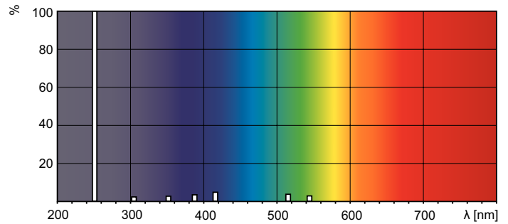
XDP0_XUTUVPLL-Spectral power distribution Colour
